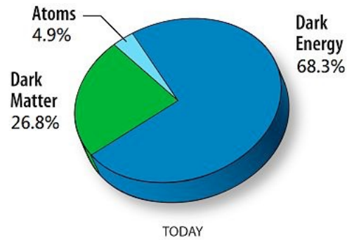
Mass and energy in the Universe
